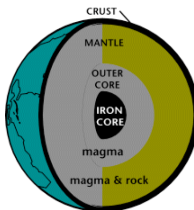
THE EARTH'S INTERIOR
